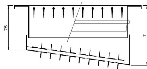
YKM-DD TYPE INCLINED HIT WITH DAMPER
