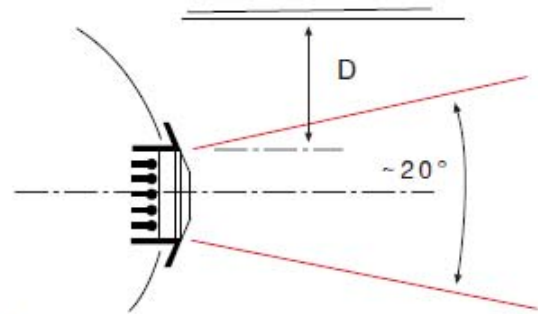
B) Without Ceiling Effect D=max.0,90m ( Correction Chart )
