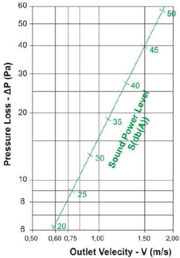
Pressure Loss and Sound Level Graph
