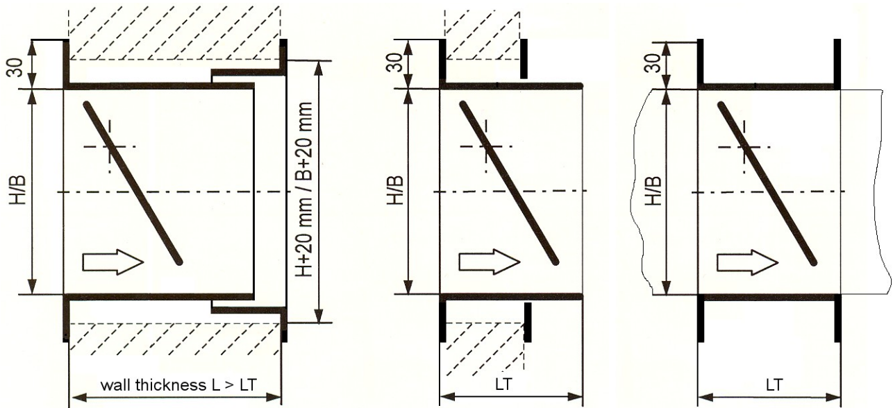
Wall form "T"
